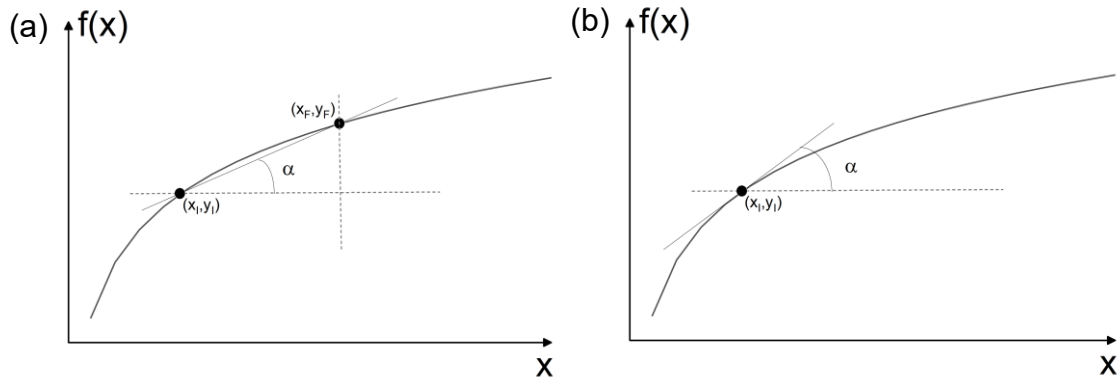
Figure 3. Sketch of the angle \alpha formed by (a) the line that passes through two arbitrary points (x_I, y_I) and (x_F, y_F) which are solutions of f(x) and a line parallel to the x axis and (b) the line tangent to (x_I, y_I) and a line parallel to the x axis.
